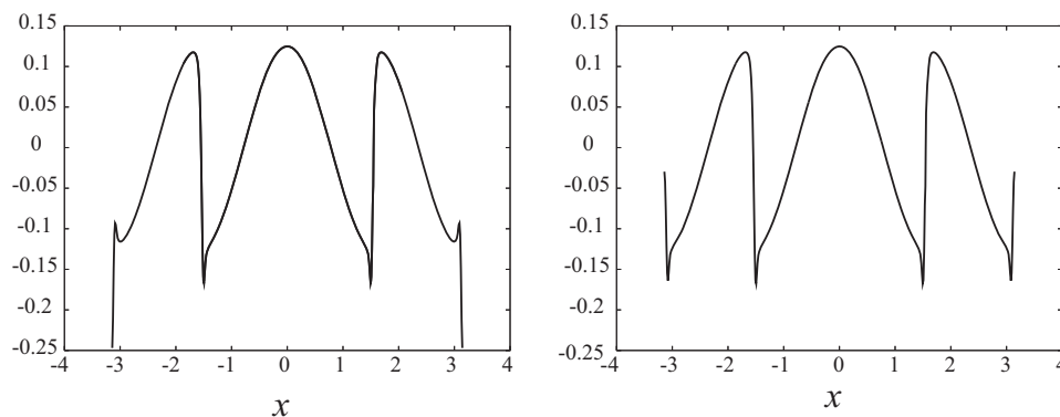
Figure 22: Graphs of two different \psi' . R = 10^4, \alpha = -3.2 .
