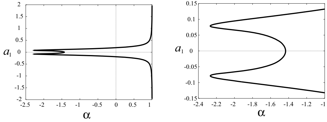
Figure 16: The bifurcation diagram: \ell = 2 . R = 100 .
