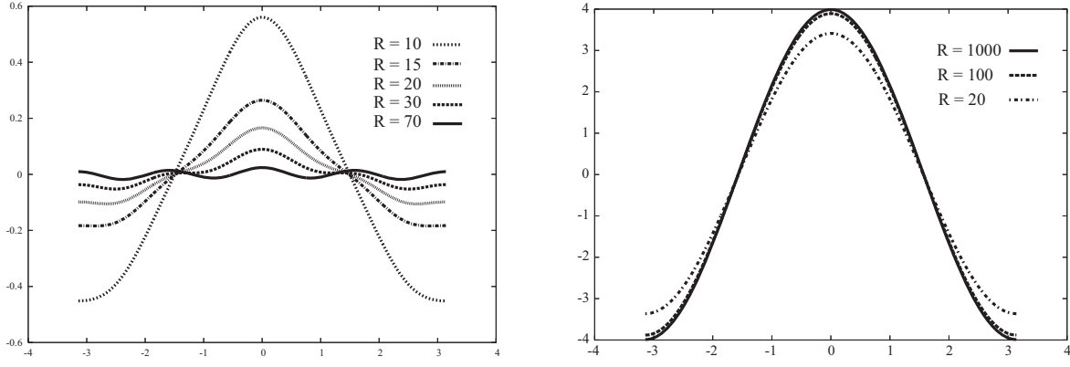
Figure 4: Profiles of \psi' . \ell = 4 . \alpha = 1 . R = 10, 15, 30, 70 (left). R = 20, 100, 1000 on uppermost branch (right). The figure on the right shows that \lim_{R \rightarrow \infty} \psi'_R = 4 \cos x .
