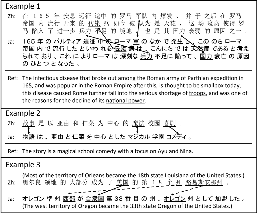
Figure 4.6: Examples of sentences additionally extracted by combining the extracted bilingual lexicons to the Baseline (example 1 and 2 are truly parallel sentences, while example 3 is an erroneous parallel sentence pair). The lexicon pairs that do not exist in the Baseline generated dictionary but extracted by our bilingual lexicon extraction method are linked (correct lexicon pairs are linked with solid lines, incorrect lexicon pairs are linked with dashed lines).
