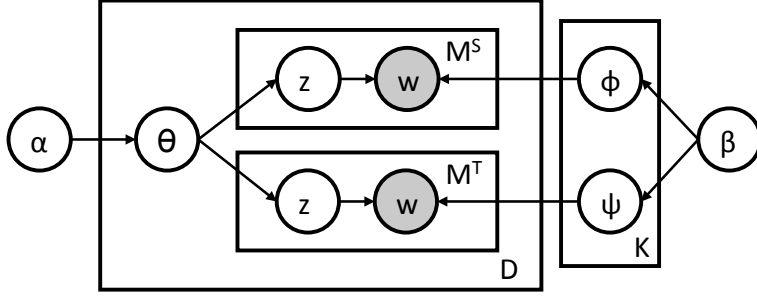
Figure 3.2: BiLDA topic model.
