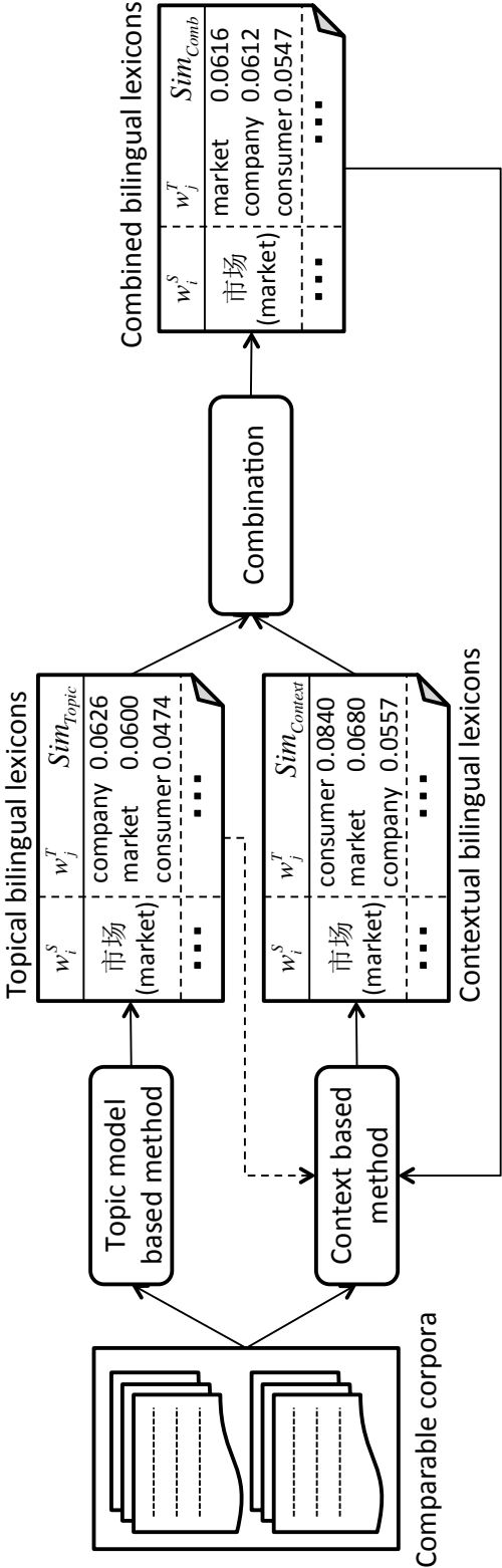
Figure 3.1: Bilingual lexicon extraction system.
