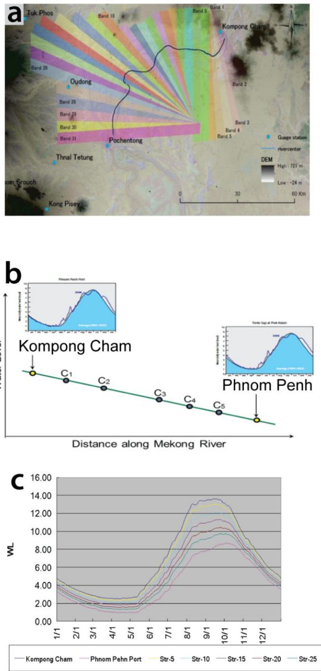
Fig. 2-12 Applying flood hydrographs to each band in the study area such as a) Division of floodplain by band, b) Interpolation of neighboring hydrographs, c) Hydrographs for each band
