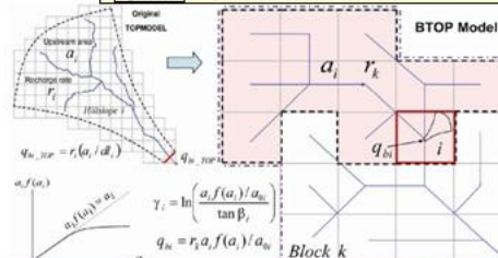
Fig 4-17 Schematic mechanism of BTOP runoff model
