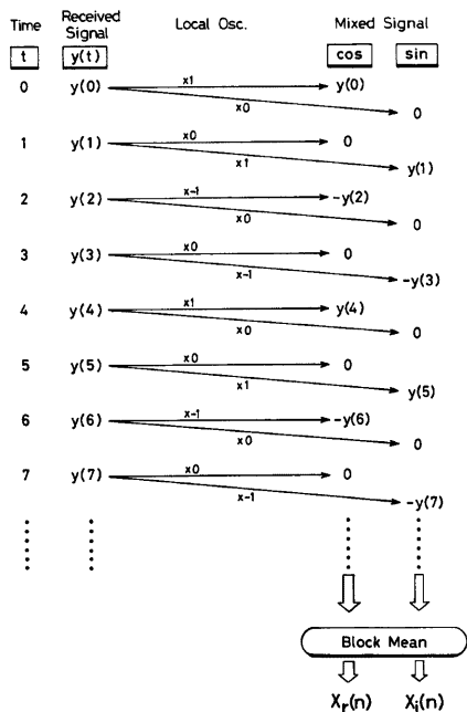
Fig. 6 Data handling process of SHCC method.
