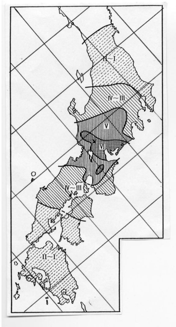
Fig.1 Seismic intensity map of the Nobi earthquake by JMA after Usami(2003). Latitudinal and longitudinal lines are written in every 2 degrees.
