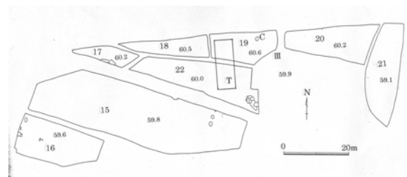
Fig.3 Division numbers of the archaeological excavation on the flood plain written the height above the sea level. T shows the division of the trench, III indicates right lateral offset and C means circle in the photographs No.4 and No.5 after Okada and Tsutsumi (1997). Figure is modified from the archeological report.
