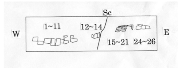
Fig.2 Arrangement of the divisions of archaeological investigations before the trench research. Sc means scarp, which divides the area into the terrace in the west and the flood plain in the east. Figure is modified from the archeological report.
