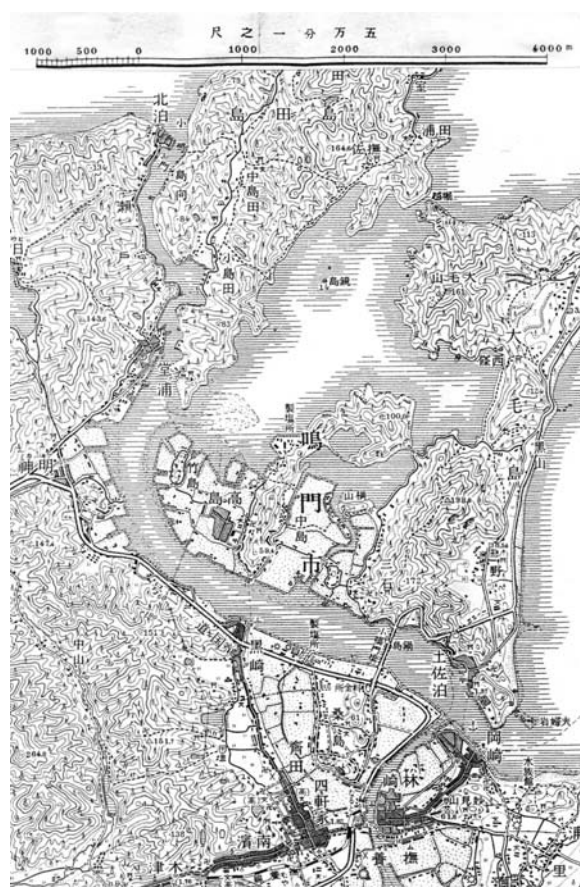
Fig.6 Topographic map around Naruto. [Naruto-Kaikyo, 1/50,000, Geographical Survey Institute (1968)]
