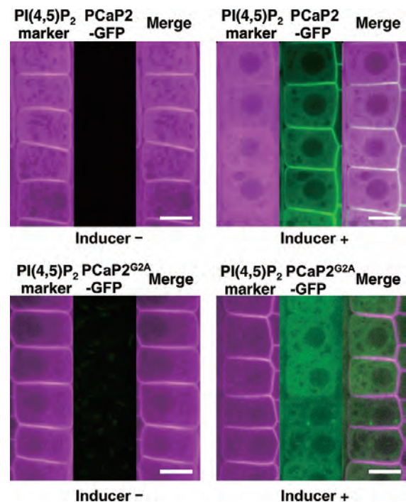
Figure 2. Fluorescence images of PCaP2-GFP (a) or PCaP2 Δ23A -GFP (b) expressed by an estradiol-inducible promoter, the PI(4,5) \text{P}_2 marker (magenta) expressed by the UBIQUITIN10 promoter, and their merged images in meristematic root epidermal cells treated with (right panels) or without (left panels) 10 \mu\text{M} \beta -estradiol for 5 hours are shown. Bars = 10 \mu\text{m} .
