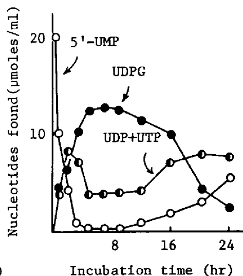
Fig. 11. UDPG Formation in the Absence of Galactose by Lactose-Grown T. candida .
