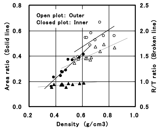
Fig. 4 Relationships among area ratio, R/T ratio, and bamboo density.
