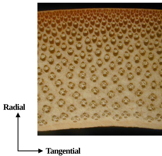
Fig. 1 Typical transverse cross-sectional features of Moso bamboo, a, and the schematic shape change in the vascular bundle from the inner to outer layers, b.
