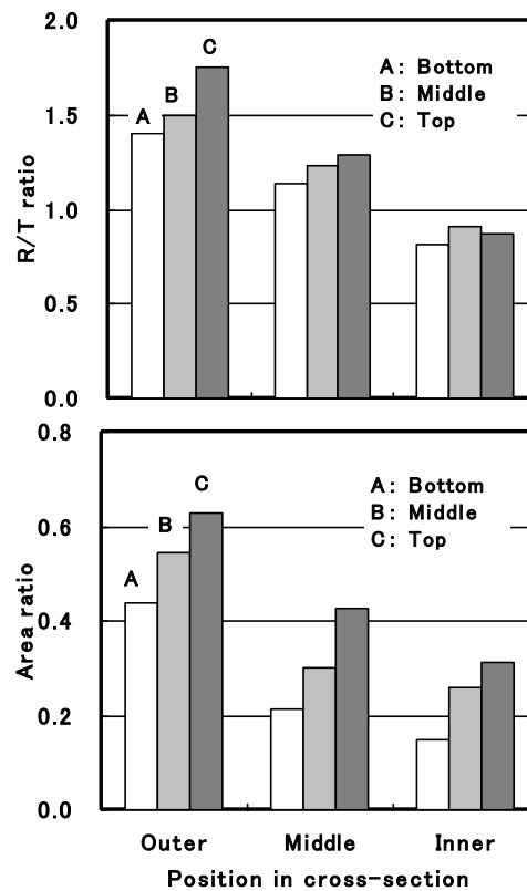
Fig. 3 Change in the vascular bundle R/T ratio and area ratio with cross-sectional position.
