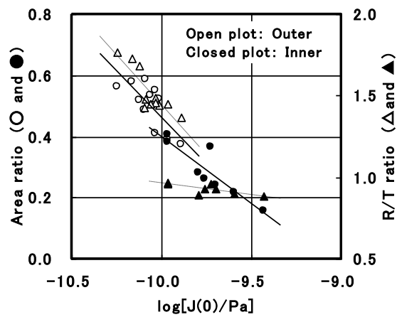
Fig. 7 Relationship between area ratio and R/T ratio and the instantaneous creep compliance J(0) .
