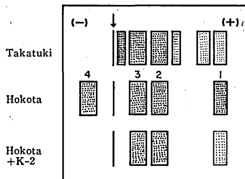
Fig. 1. Esterase zymograms of houseflies. K-2 ( 10^{-5} M) was incubated with enzyme solution for 30 min. at 0^{\circ}\text{C} before electrophoresis.
