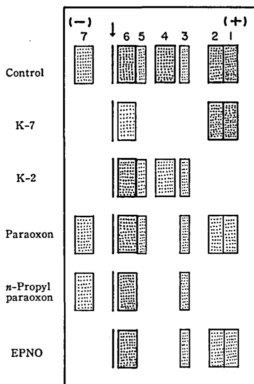
Fig. 2. Effect of organophosphorus esters on esterase zymograms for G strain. Inhibitors were incubated with enzyme solution for 30 min. at 0^{\circ}\text{C} before electrophoresis. K-7: 10^{-5} M. K-2, paraoxon, n -propyl paraoxon and EPNO: 10^{-5} M.
