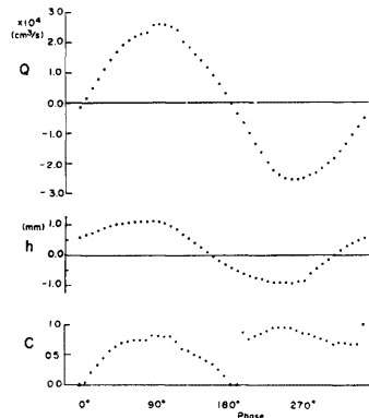
Fig. 10. Rate of flow through Takahama Straits ( Q ), difference of water level between Stn. A and Stn. D ( h ), and coefficient of rate of flow ( C ).
