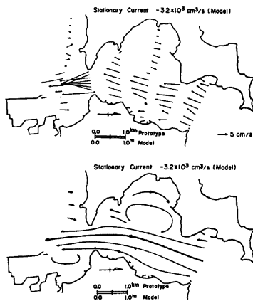
Fig. 9. Flow pattern in the case of southward stationary current corresponding to the ebb tidal one.
