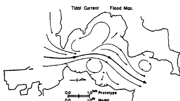
Fig. 6. Flow pattern at the flood.
