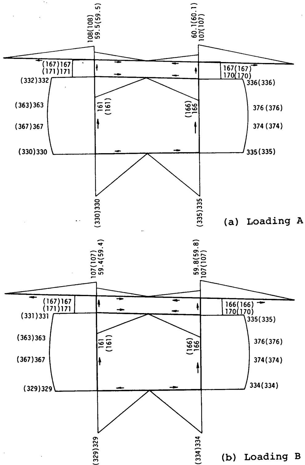
Fig. 4.17 Shear Flows Due to Bending Moment M_y
