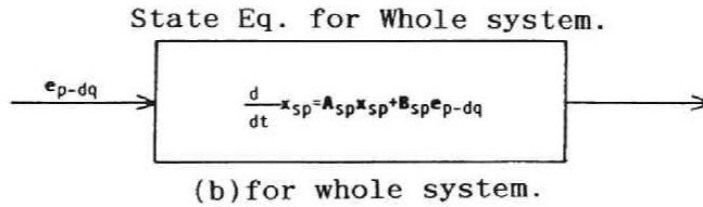
Fig.3-3 State equations (a)divided into i) for SMES side and ii)for power system side (b)for whole system.
