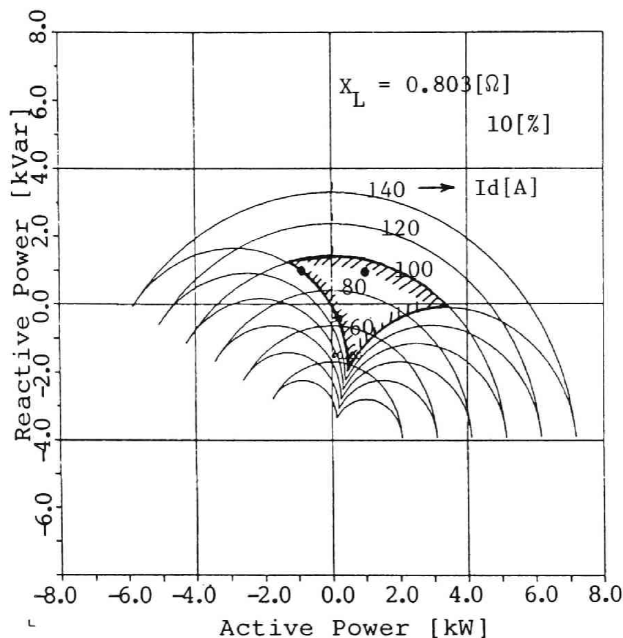
Fig.4-12 P-Q characteristics with designed filters and possible region for P-Q simultaneous control (shaded region; I_d 100[A]-140[A])
