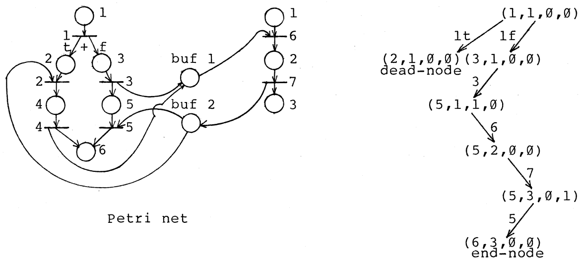
Figure 7. An example of deadlock.
