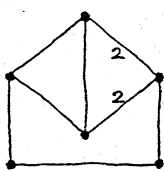
\sim^d G(6,8;6-a_5)
