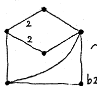
10_{69}
