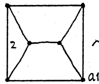
10_{121}
