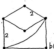
self-dual
