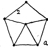
10_{113}
