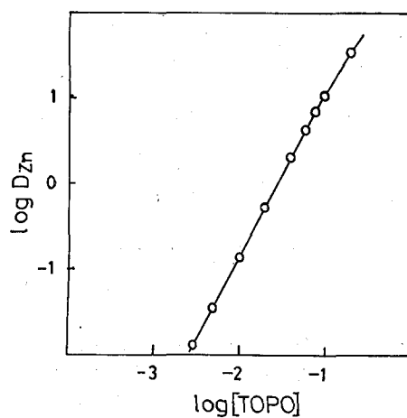
Fig. 6. The plot of \log D_{Zn} vs. \log [TOPO] in E.G.-toluene system.
