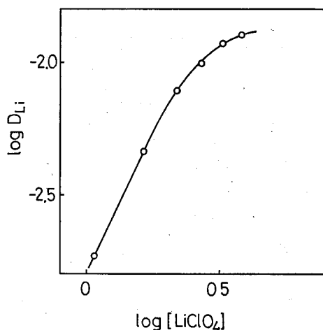
Fig. 3. The plot of \log D_{Li} vs. \log [LiClO_4] in E. G.-toluene system.
