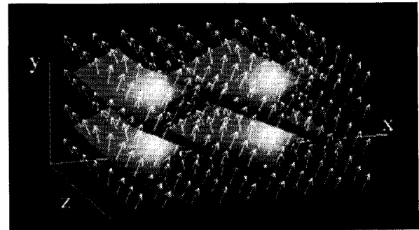
FIGURE 2. Snapshot of the TGB layer structure at \alpha = 50^\circ . Shown are the isosurface \text{Re}(\Psi) = 0 and the director in arrows.
