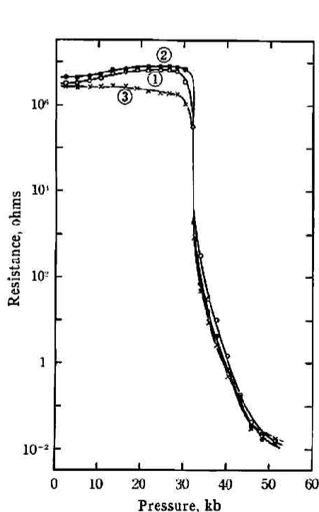
Fig. 4 Resistance versus pressure behavior of CdTe during three cycles of compression (① \rightarrow ② \rightarrow ③)
