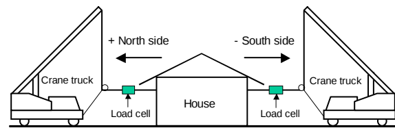
Fig. 5 Static cyclic loading test using two crane trucks
