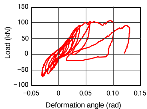
Fig. 7 Experimental result of restoring force
