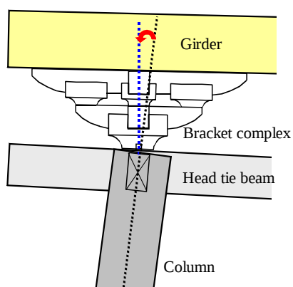
Fig. 18 Rocking of column and bracket complex
