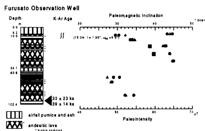
Fig. 3 Geological column and paleomagnetism of the Furusato observation well, Sakurajima volcano.
