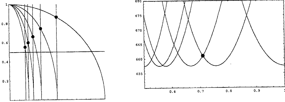
Figure 5: Pseudo hexagonal points of (n, 1) and (n + 1, 0) (left) and the vertical section of neutral critical surfaces on the line \{(\alpha, \beta) = sk_c(1/2, \sqrt{3}/2); s \in (1/2, 1)\} (right). Each curves in the right figure corresponds to the section of S_{1,1}, S_{2,1}, S_{3,0}, S_{3,1}, S_{1,2} and S_{2,2} from the right, respectively. Notice that the pair of surfaces \{S_{1,1}, S_{2,0}\} as well as \{S_{0,2}, S_{3,1}\} coincide each other on this line. Black dot is the point where the patchwork-quilt is stable.
