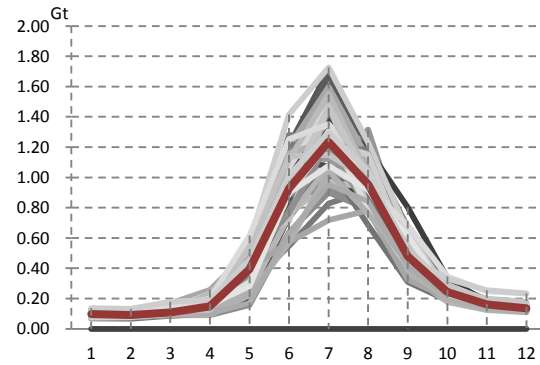
Fig. 5 Average water balance for whole year ensemble (1972-2000)
