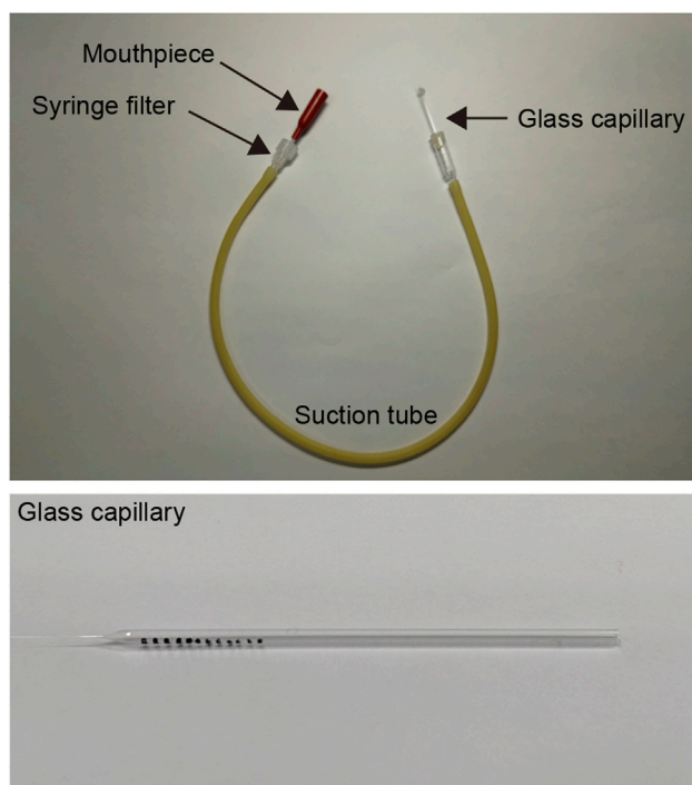
Figure 2. Mouth-controlled micropipette
