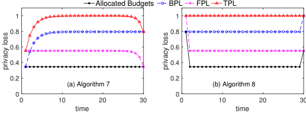
Fig. 8. Privacy Budget Allocation Schemes for 1-DP T .
