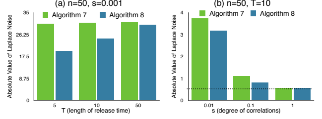
Fig. 9. Data utility of 2-DP T mechanisms.
