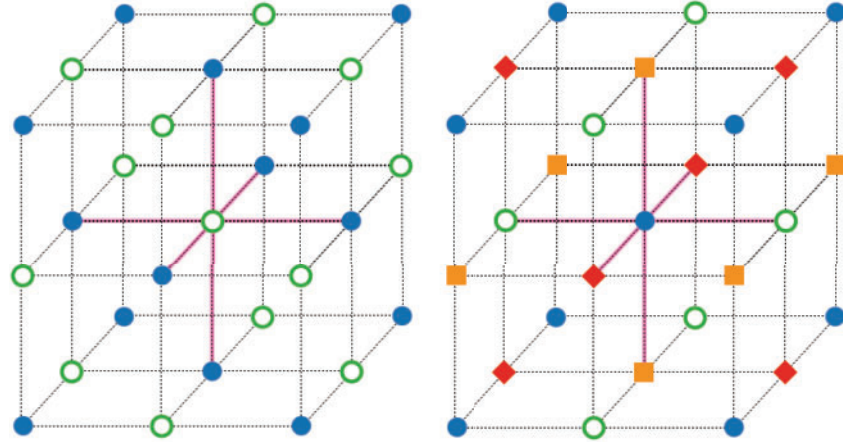
Fig. 1. Schematic figures of s2 dilution (left) and s4 dilution (right). Sites with different symbols belong to different diluted noises. Pink lines connect sites that are referred to in the calculation of the Laplacian at the central point.
