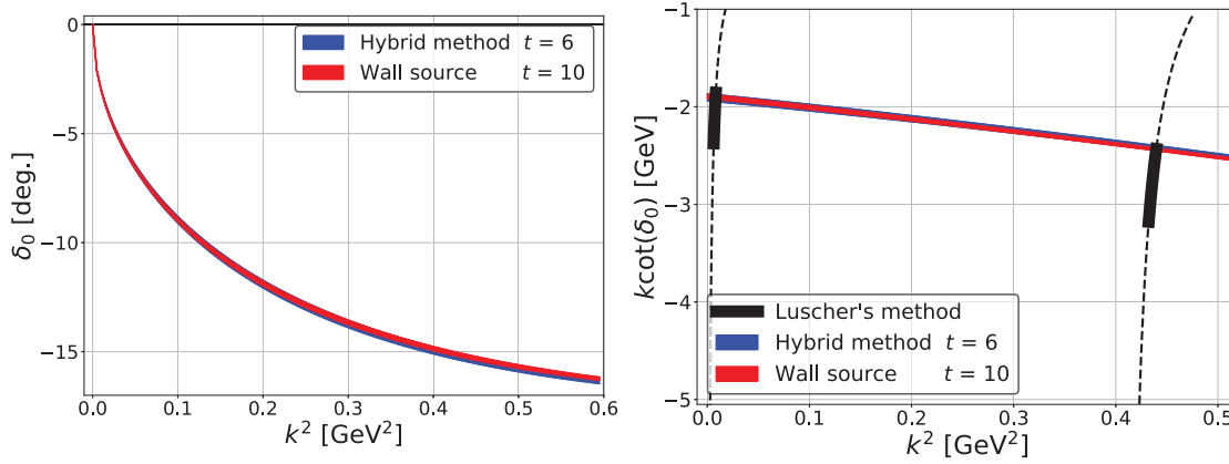
Fig. 10. (Left) Scattering phase shifts \delta_0(k) as a function of k^2 . (Right) k \cot \delta_0(k) as a function of k^2 . Blue (red) bands correspond to the results from the HAL QCD method with the hybrid method (with the wall quark source). Black bands in the right figure correspond to the results from Lüscher's method [34].
