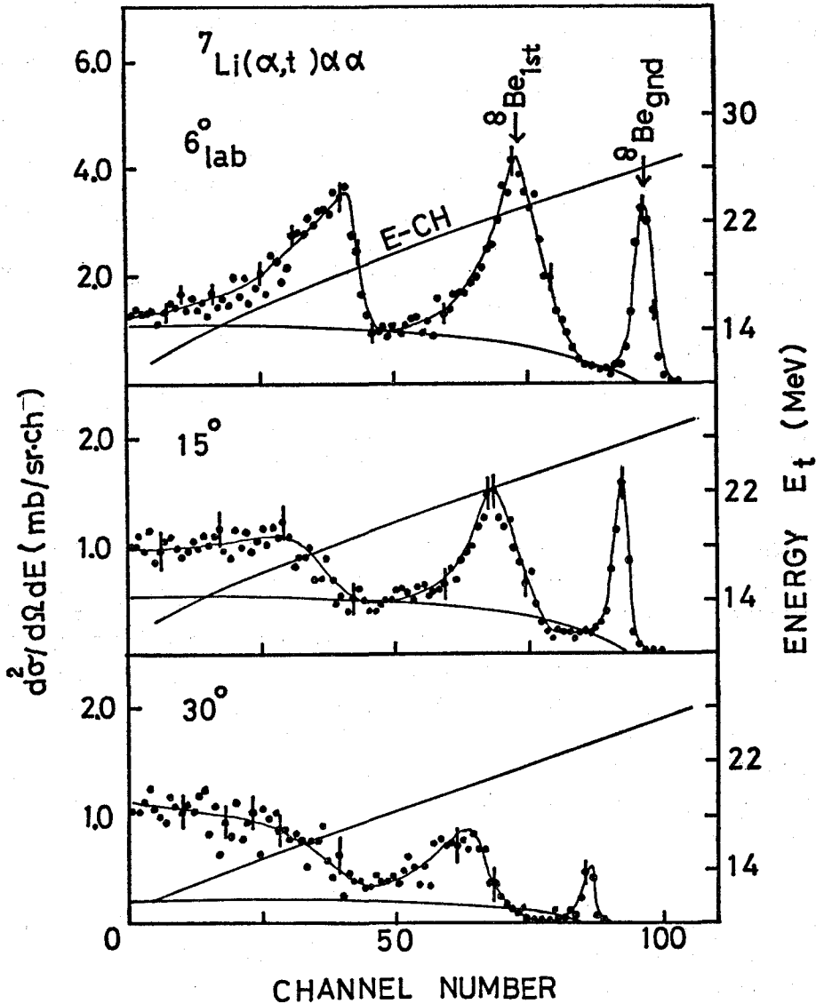
Fig. 13-5. Energy spectra of tritons at 6°, 15°, and 30° (lab) from the {}^7\text{Li} + \alpha reaction with 29.4 MeV alpha particles. Typical error bars are shown. The curve labelled E-CH gives the relation between particle energy and channel number. The smooth curves are the prediction of the phase space factor. From [74-8].
