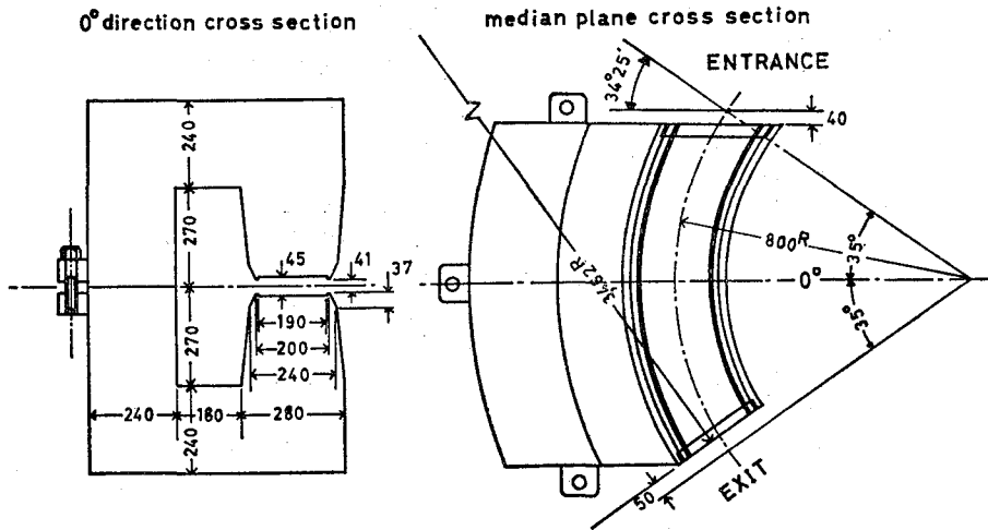
Fig. 7-2. Dimensions of the beam momentum analyzing magnet. From [69-9].
