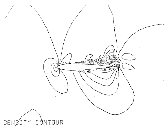
Fig.8 M=0.75 , Re=10^5 , T=24 .
