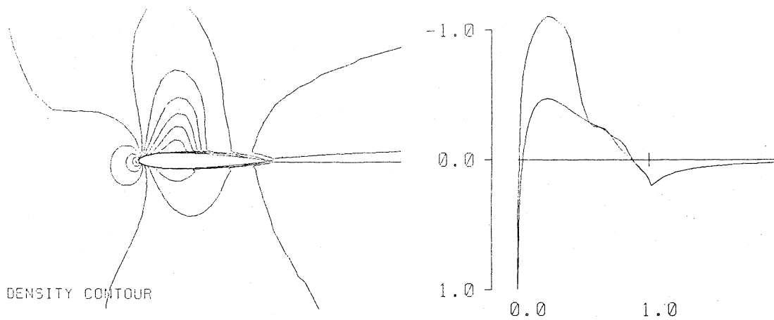
Fig.11 M=0.75 , Re=10^5 , Baldwin-Lomax turbulence model, 81x41 mesh-points.
