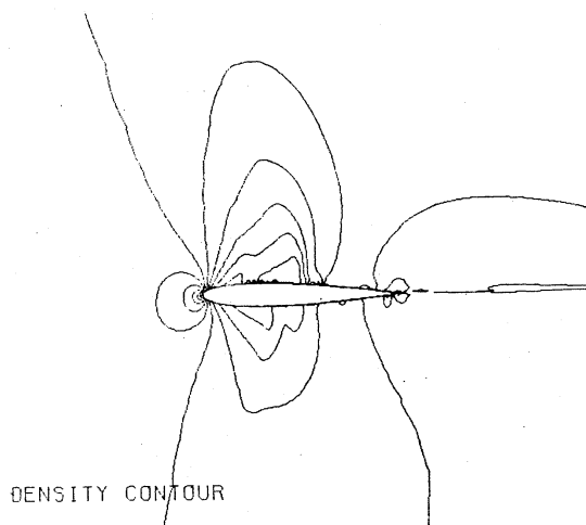
Fig.13 M=.75 , Re=6.7 \times 10^6 , T=5 .
