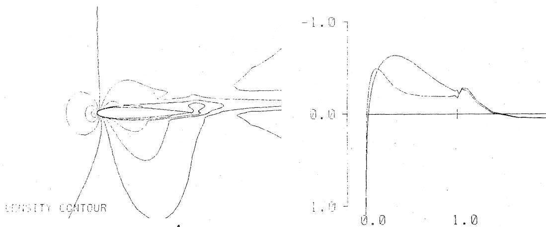
Fig.12 M=0.75 , Re=10^4 , 81x41 mesh-points.
