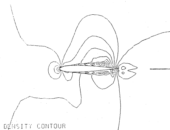
Fig.9 M=0.75 , Re=10^5 , T=31 .
