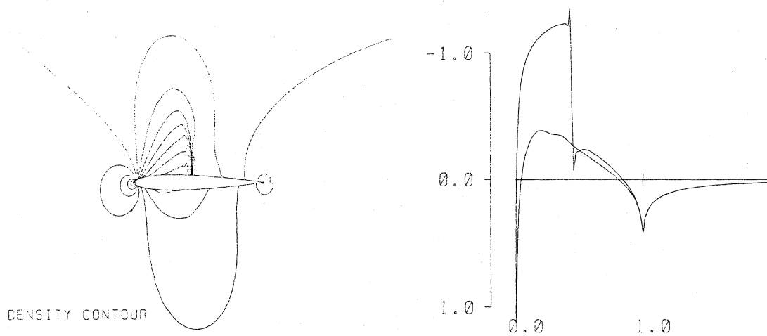
Fig.10 M=0.75 , inviscid flow.
