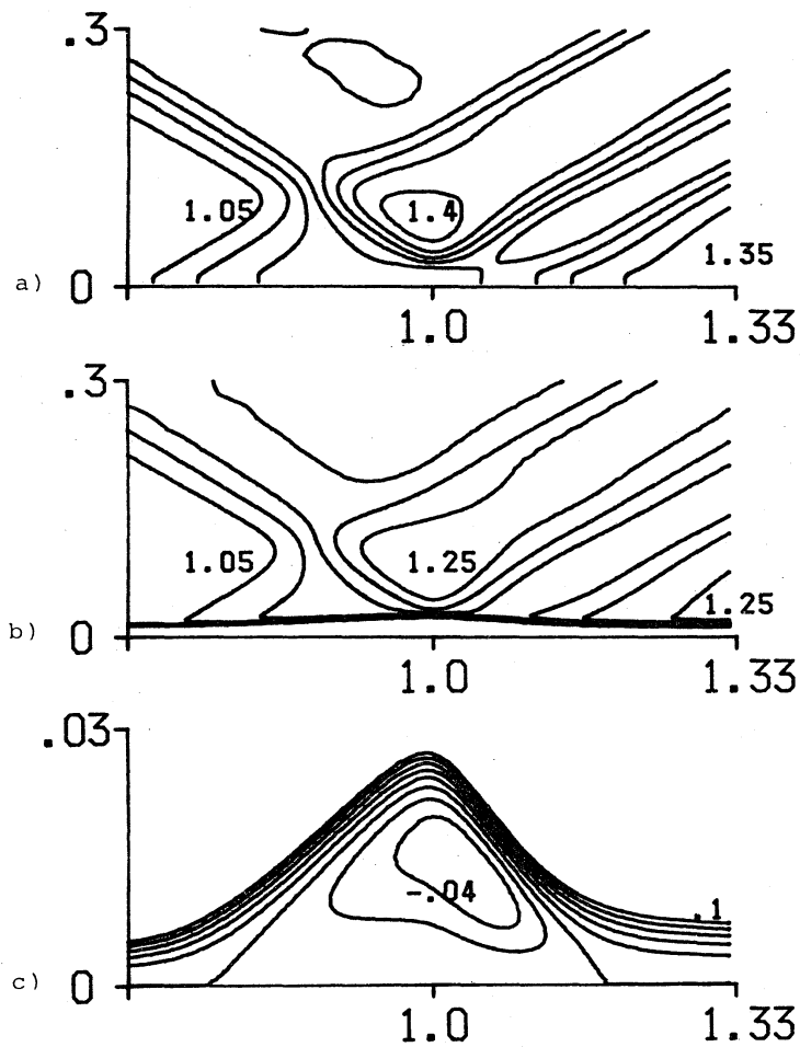
Fig.5 Numerical contour maps near the incident point of shock wave for 256x96 mesh-points.
