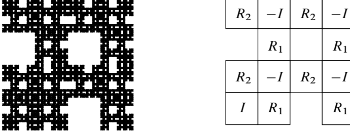
Figure 4.3. Non-countably ramified example.
