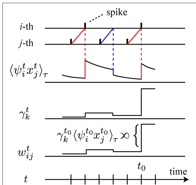
FIGURE 1 | Schematic illustration of the learning rule. For simplicity, we illustrate only the relation between \langle \psi_i^t x_j^t \rangle_\tau , \gamma_k^t and w_{ij}^t , omitting the other components of the learning rule. On the first two lines, spikes of the i -th and the j -th neurons are depicted. On the third line, \langle \psi_i^t x_j^t \rangle_\tau decays with time constant \tau , and is modulated by the interactions between the spiking activity of the i -th and the j -th neurons. When the firing of the presynaptic j -th neuron precedes the firing of the postsynaptic i -th neuron, \langle \psi_i^t x_j^t \rangle_\tau increases (red line). If the postsynaptic neuron fails to fire, \langle \psi_i^t x_j^t \rangle_\tau decreases (blue line). The change of the synaptic weight w_{ij} at time t_0 is proportional to the product of the amount of global signal \gamma_k^{t_0} and \langle \psi_i^{t_0} x_j^{t_0} \rangle_\tau as depicted on the fifth line.
