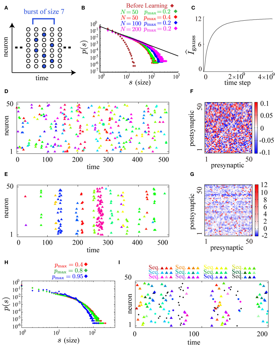
FIGURE 3 | Neuronal avalanches are reproduced by applying the learning rule to spontaneously firing recurrent neural networks. (A) A schematic illustration of the definition of bursts and their sizes. A burst of size 7 that lasts for 3 time steps is illustrated in the figure. (B) Log-log plots of burst size s against the occurrence of bursts of that size p(s) before (brown) and after learning (red for p_{\max}=0.4 and N=50 , green for p_{\max}=0.2 and N=50 , blue for p_{\max}=0.2 and N=100 , and magenta for p_{\max}=0.2 and N=200 ). The size distributions after learning fall on the straight line of slope around -3/2 (the black line). (C) The approximate measure of the mutual information \hat{I}_{\text{gauss}} is calculated during the course of learning. (D,E) Typical raster plots before (D) and after (E) learning in which spikes belonging to different bursts are displayed in different colors. (F,G) Connection weight matrices of the network before (F) and after (G) learning in which rows correspond to connections to single postsynaptic
