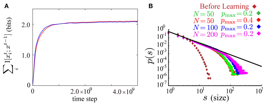
FIGURE 6 | (A) Time evolution of the sum of the neuron-wise information terms \sum_i I[x_i^t; x^{t-1}] during the course of learning according to the objective function with the lower bound A_1 , Equation (9) (the red curve), and the modified objective function obtained by replacing A_1 with A'_1 , Equation (10) (the blue curve). (B) The results in Figure 3B are reproduced after learning with the modified objective function and the same learning
