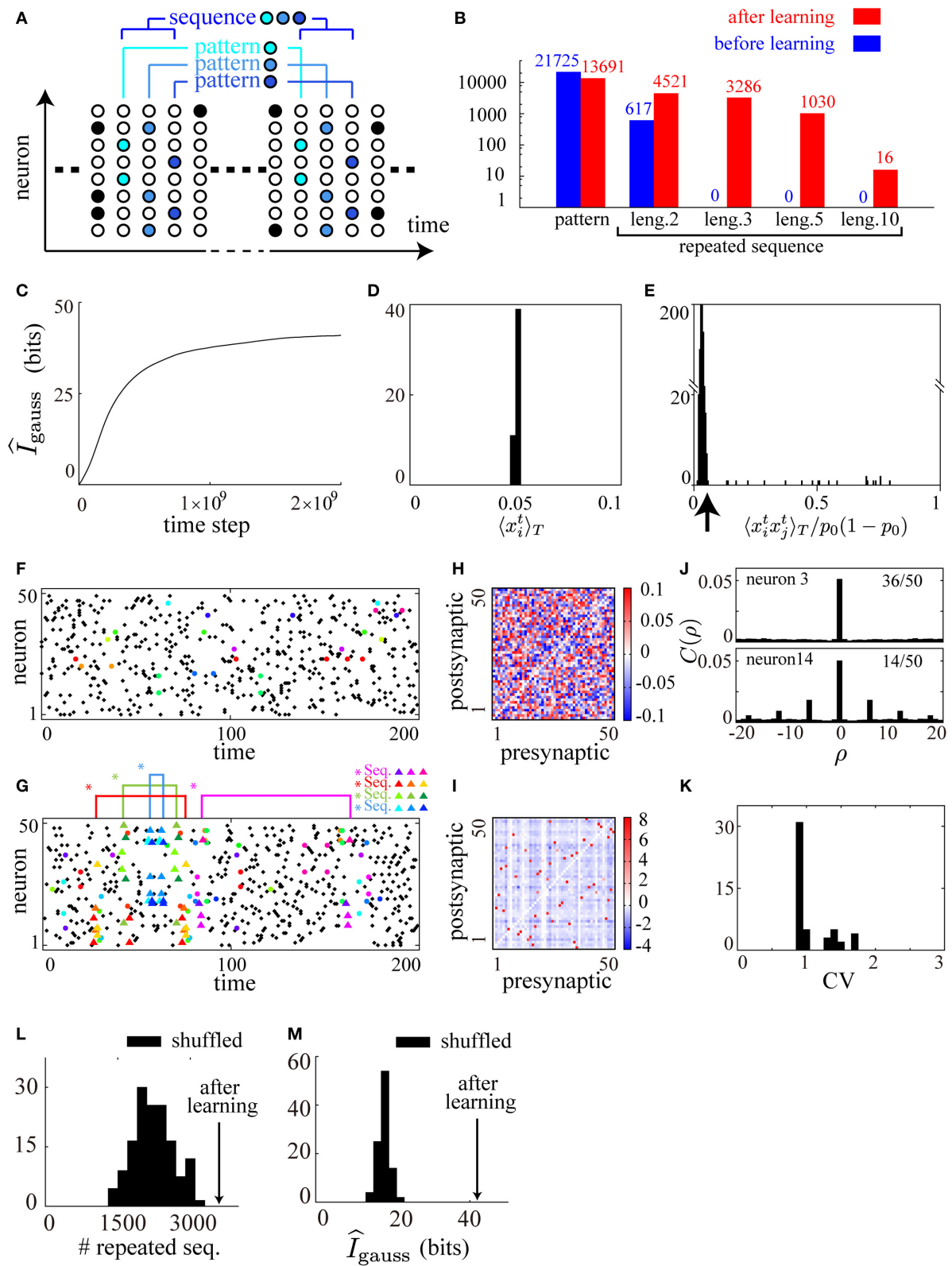
FIGURE 2 | Cell-assembly-like repeated sequences of firing patterns are reproduced by applying the learning rule to a spontaneously firing recurrent neural network. (A) A schematic illustration of the definition of
