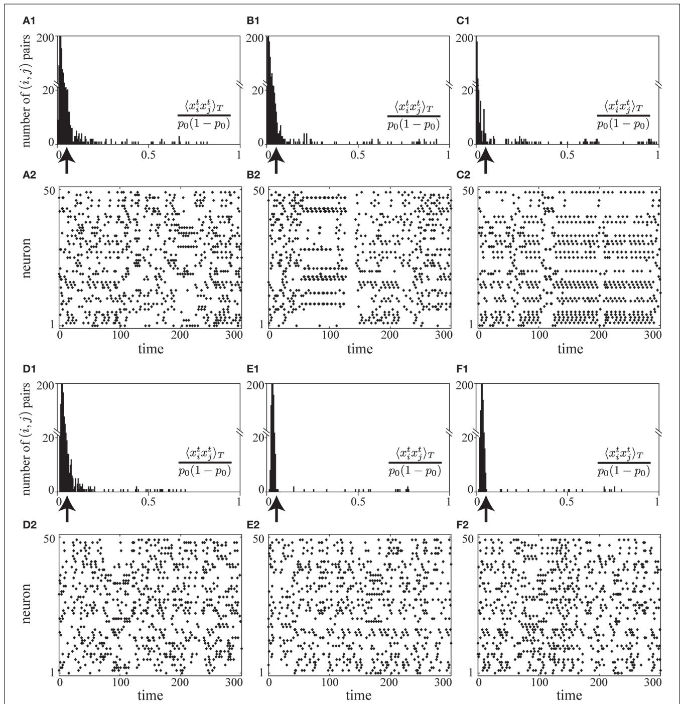
FIGURE 7 | (A1–C2) A simulation of learning in a spontaneously firing network without the fluctuation term A_4 . Histograms of pairwise correlations \langle x_i x_j \rangle_T / \{p_0(1 - p_0)\} ( i \neq j ) ( A1–C1 ) and raster plots ( A2–C2 ) at different time steps during learning (the 5 \times 10^8 , 1 \times 10^9 , and 2 \times 10^9 -th steps, respectively) are shown. The learning coefficient c_\zeta is set to be 10000.0 so that the fluctuation term A_4 does not take effect. ( D1–F2 ) A simulation of learning in a spontaneously firing network under the effects of the fluctuation term A_4 . Histograms of pairwise correlations \langle x_i x_j \rangle_T / \{p_0(1 - p_0)\} ( i \neq j ) ( D1–F1 )
