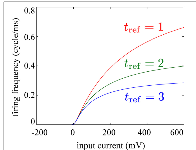
FIGURE 8 | Dependence of firing frequencies of an integrate-and-fire model on magnitudes of constant input currents falls on a sigmoid curve. Saturating frequencies depend on the length of the refractory period t_{\text{ref}} as indicated by the differently-colored curves [red: t_{\text{ref}} = 1 (ms), green: t_{\text{ref}} = 2 (ms), blue: t_{\text{ref}} = 3 (ms)].
