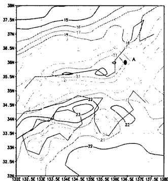
Fig. 5 Distribution of temperature from GPV on 925hPa.
