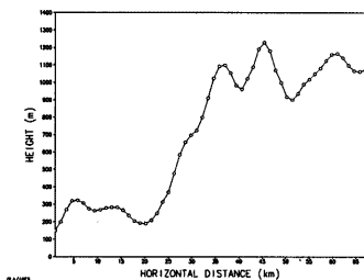
Fig. 4 Topography smoothed by Low Path Filter.
