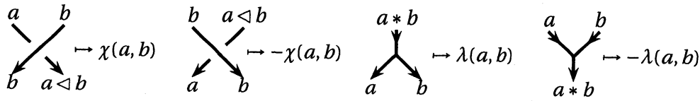
Figure 8: Qualgebra 2-cocycle \leadsto weight
