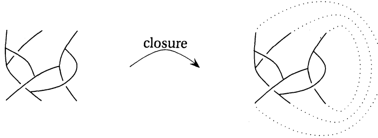
Figure 11: Branched braid \leadsto 3-graph
