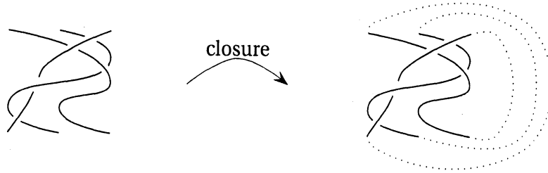
Figure 9: Braid \leadsto link
