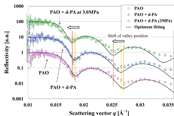
Fig. 1 Reflectivity profiles obtained from the interface in PAO (bottom), in PAO with deuterated palmitic acid (d-PA) (middle), and in PAO with d-PA at 3.0 MPa (top).
