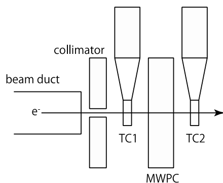
Fig. 1 Experimental Setup
