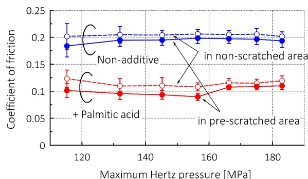
Fig. 2 Coefficients of friction measured with SiO 2 colloidal probe in hexadecane without/with palmitic acid in pre-scratched area and outside area.
