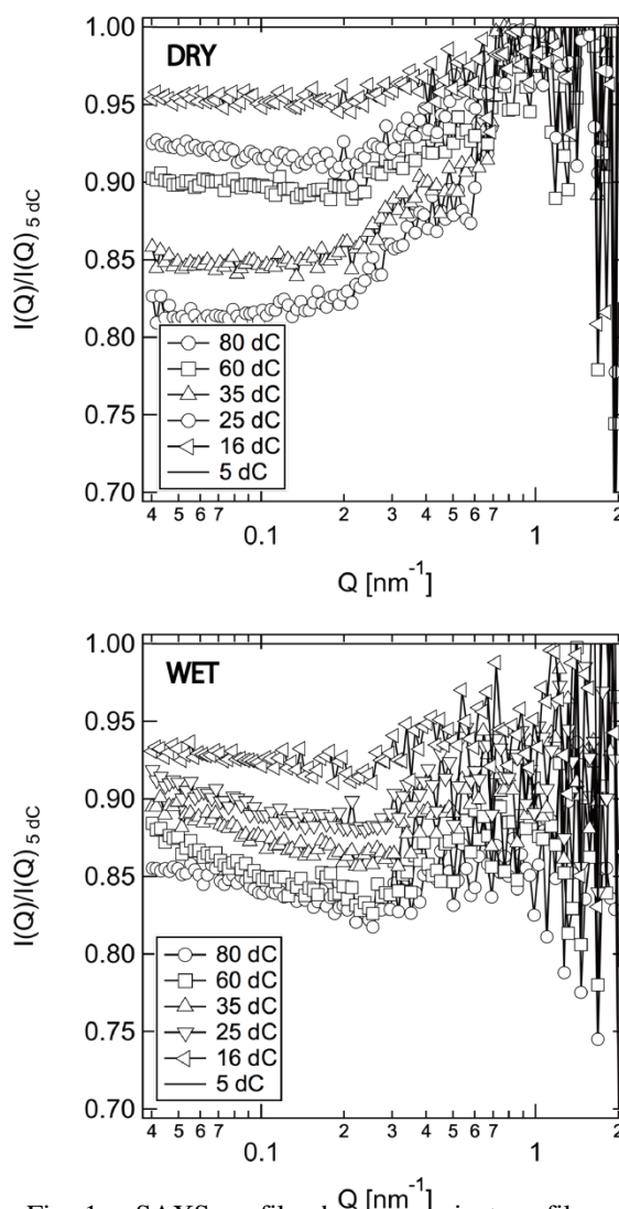
Fig. 1. SAXS profile changes against profiles of 5 dC under dried and wet conditions.
