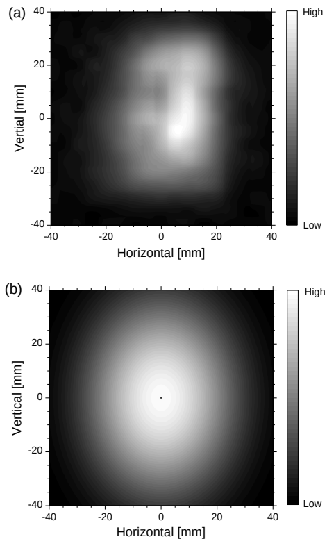
Fig. 1 Measured (a) and calculated (b) two-dimensional distributions of the CCR-MCP.
