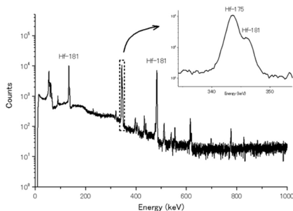
Fig. 2. Gamma-ray spectrum of hafnium oxide film + spike solution (HfO 2 +Sp).
