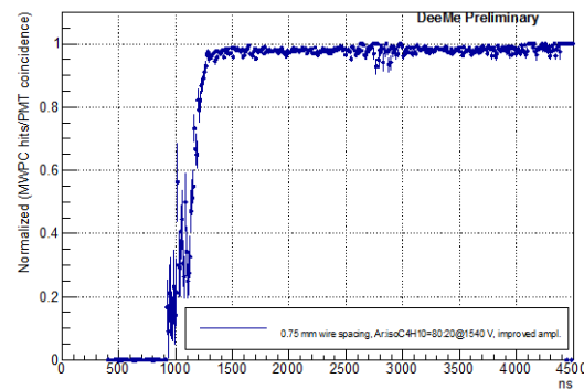
Fig. 2 Efficiency of the high-voltage switching MWPC as a function of time. Time origin corresponds to the time of high-voltage gate.
