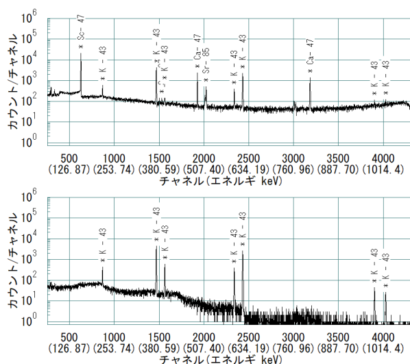
Fig. 1. Gamma-ray spectra of ^{43}\text{K} before (upper) and after (lower) purification.
