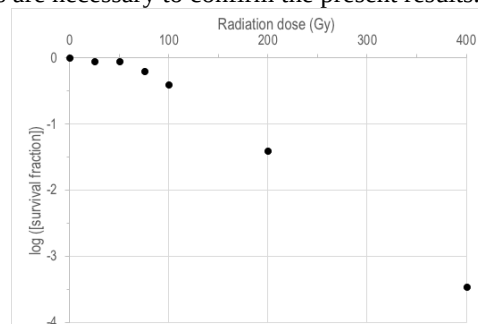
Fig. 2. The radiation survival fraction curve of Bacillus subtilis natto.
