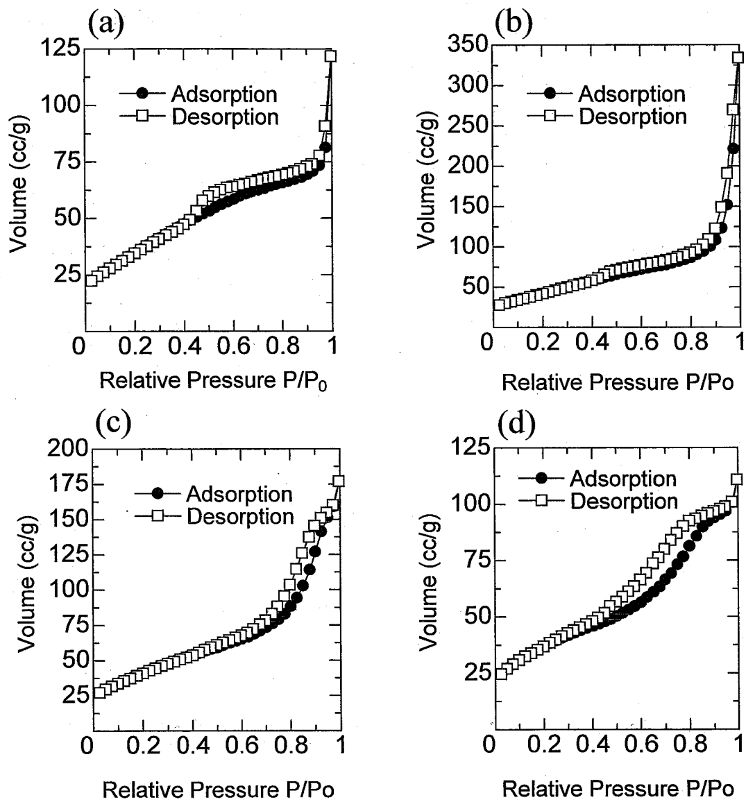
Fig. 3-12. Nitrogen adsorption isotherms of: (a), \text{Gd}_2\text{O}_3(400) ; (b), \text{Dy}_2\text{O}_3(400) ; (c), \text{Er}_2\text{O}_3(400) ; and (d), \text{Yb}_2\text{O}_3(400) .
