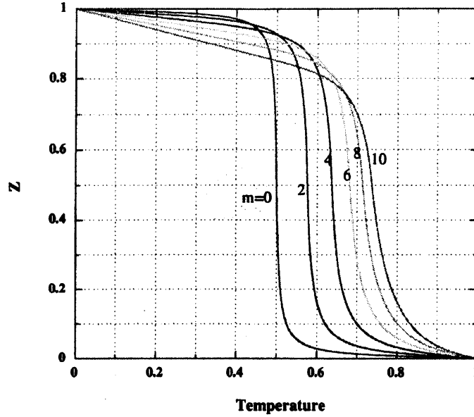
Fig 3: Horizontal mean temperature profile in convective layer with strongly temperature dependent viscosity. m is indicator of temperature dependency of viscosity
