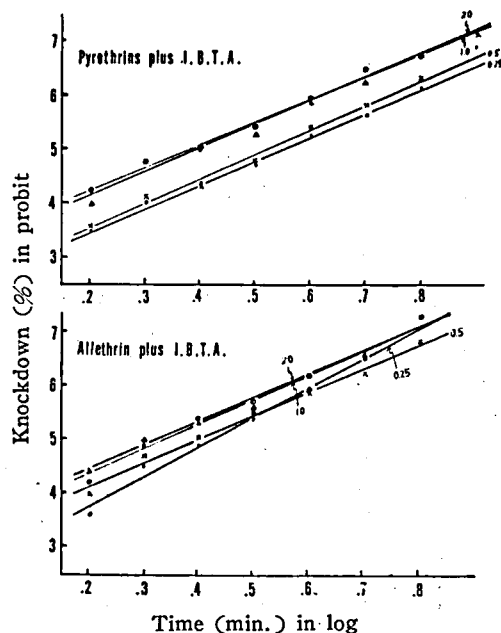
Fig. 3. The relation between time and percent knockdown of adults of the common house fly, for either pyrethrins or allethrin plus isobornyl thiocynoacetate.
