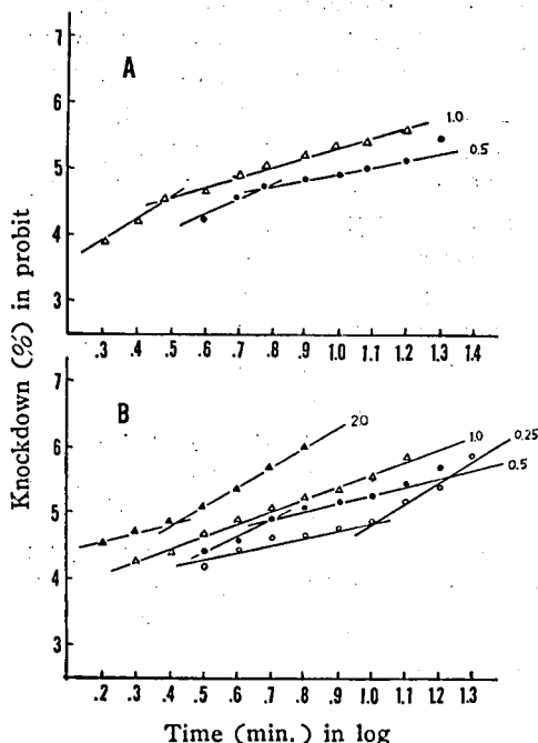
Fig. 4. The relation between time and percent knockdown of adults of the common house fly, for 0.25, 0.5, 1.0 and 2.0% isobornyl thiocyanacetate kerosene solution. A: 0.2ml., B: 0.3ml. respectively in sprayed volume.
