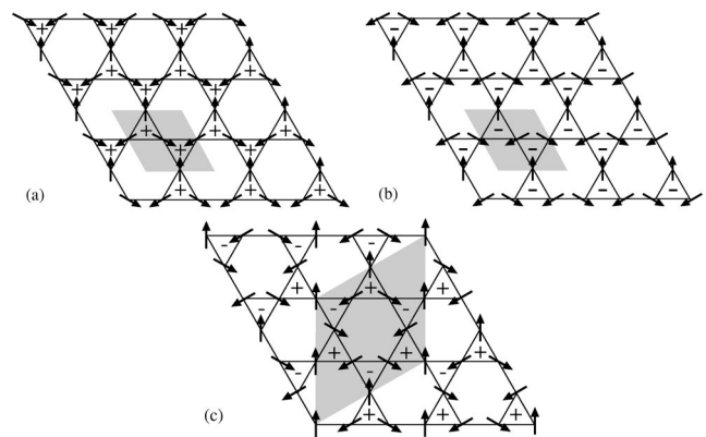
FIG. 1. Three possible Néel states of the kagomé lattice antiferromagnet: (a) \mathbf{q}=0 type with +1 chirality, (b) \mathbf{q}=0 type with -1 chirality, and (c) \sqrt{3}\times\sqrt{3} type. Plus and minus signs indicate the chirality of spins on the elemental triangles. The shaded areas indicate the magnetic unit cells.
