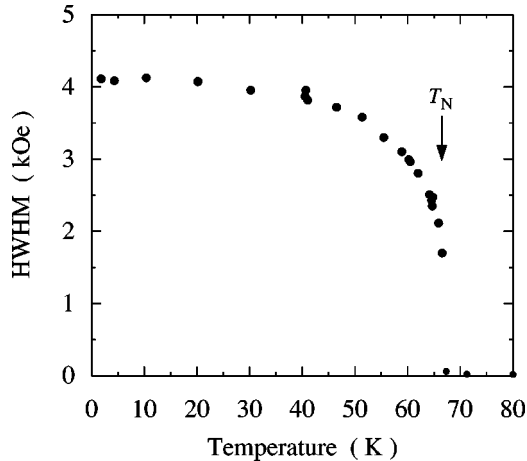
FIG. 3. Temperature dependence of the half width at half maximum of ^1\text{H} NMR spectra at 75.1 MHz.
