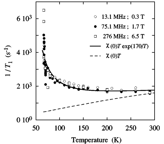
FIG. 5. Spin-lattice relaxation rate at various frequencies in the paramagnetic phase. A broken line indicates the temperature dependence of \chi(0)T . A solid curve indicates 1/T_1 \propto \chi(0)T \exp(170/T) .
