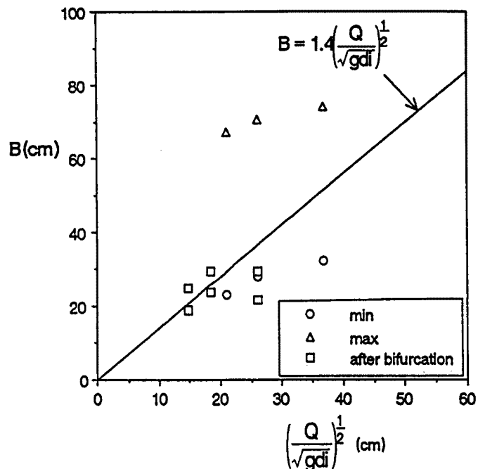
Fig. 12. Relationship between flow discharge and flow width.
