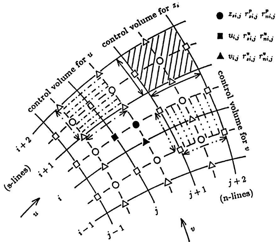
Fig. 13. Staggered locations and control volumes for velocities and water surface elevation.
