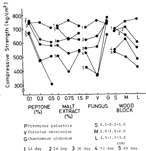
Fig. 2. Effect of factors in Experiment I using Fagus crenata (Based on the compressive strength of wood after decay).
