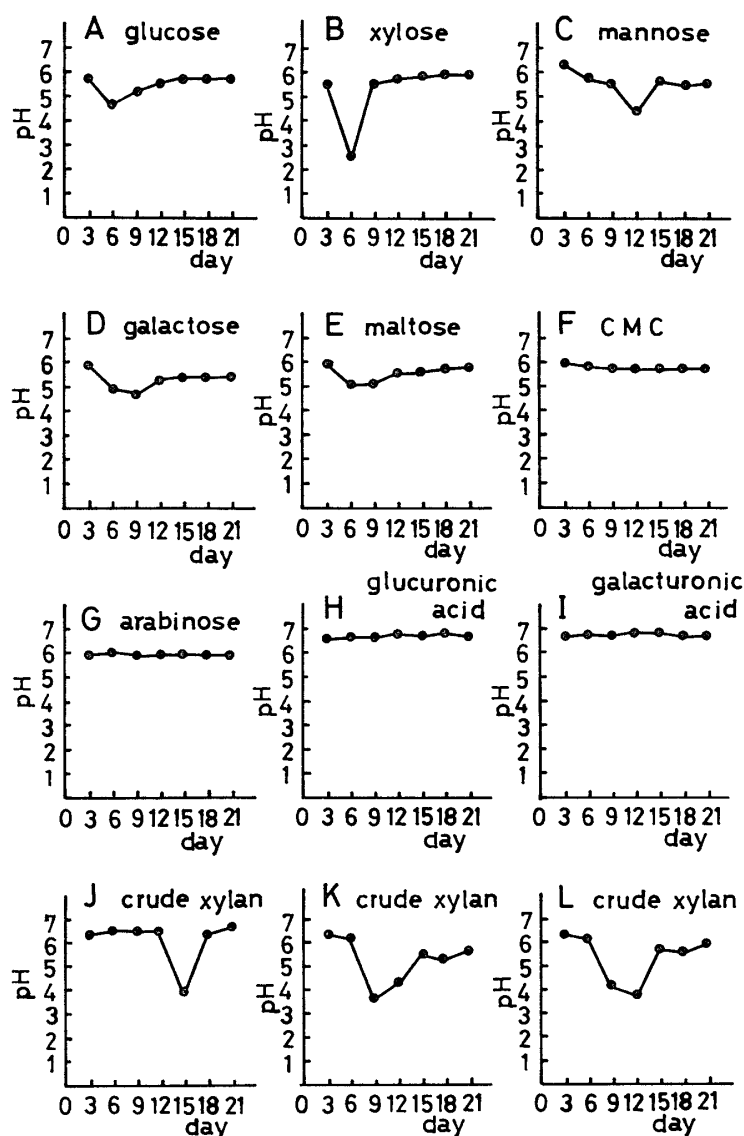
Fig. 13. Change in pH value of Abrams's medium with various carbon sources during incubation (A-J: Chaetomium globosum , K: Coriolus versicolor , L: Tyromyces palustris ).
