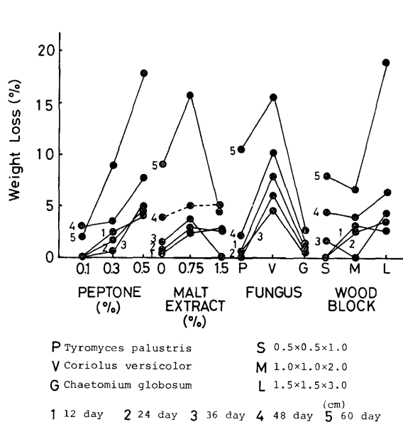
Fig. 3. Effect of factors in Experiment I using Cryptomeria japonica (Based on the loss of weight in wood after decay). Dotted line represents the non-significance at 1 and 5% levels.
