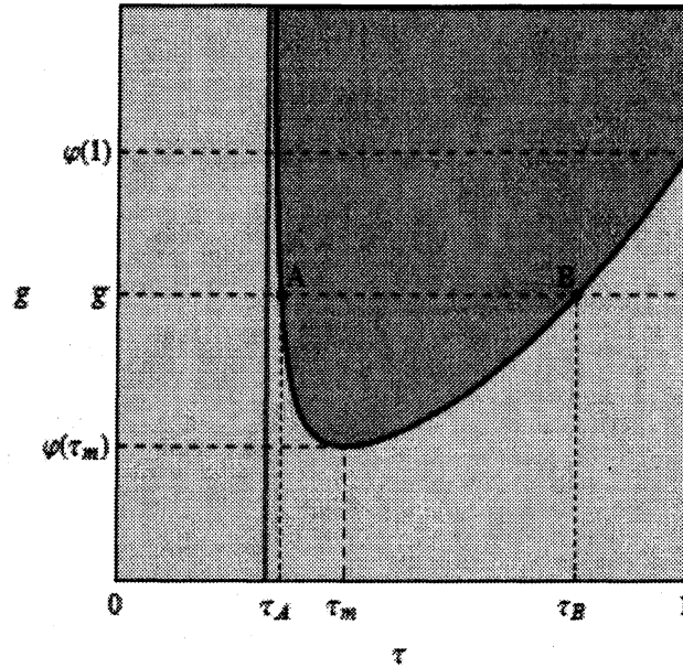
Figure 1. Stable and unstable regions
