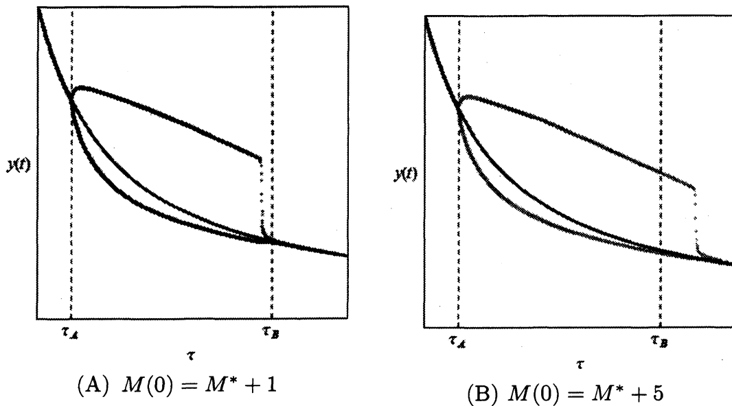
Figure 2. Bifurcation diagrams with different initial values
