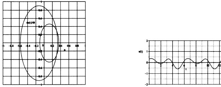
Figure 3.5: (left):The \omega(= 2\pi) -periodic solution's orbit with the initial condition: u(0) = \frac{3}{10}, \dot{u}(0) = \frac{3}{10} in Example 3.3. (right):The time histories shown up to two periods.
