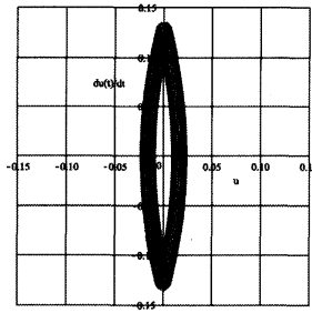
Figure 3.4: The quasi-periodic orbit with the initial condition: u(0) = 0, \dot{u}(0) = -0.12 in Example 3.2. The orbit is shown up to t = 30 .
