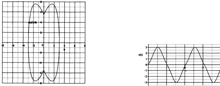
Figure 4.4: (left):The “single-time oscillation” orbit with the initial condition: u(0) = 0, \dot{u}(0) = \sqrt{30} in Example 4.1. \omega \doteq 2.047 . (right): The time history of the “single-time oscillation” orbit. The time is shown up to two periods.
