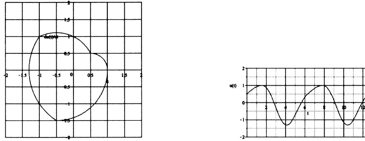
Figure 3.2: (left):The phase portrait of the hidden( 2\pi ) periodic solution in the initial condition: u(0) = \frac{1}{2}, \dot{u}(0) = \frac{1}{2} in Example 3.1. (right): The time history of the hidden( 2\pi ) periodic solution. The time is shown up to two periods.
