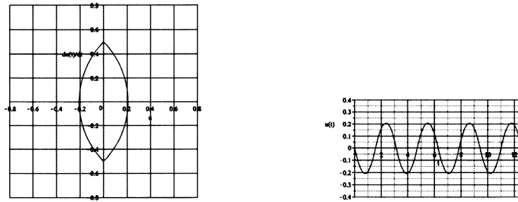
Figure 3.1: (left):The phase portrait of the \omega(=\pi) -periodic solution in the initial condition: u(0) = 0, \dot{u}(0) = -\frac{1}{2} in Example 3.1. (right): The time history of the \omega(=\pi) -periodic solution. The time is shown up to four periods.
