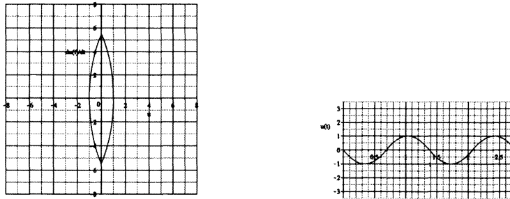
Figure 4.1: (left):The “single-time oscillation” orbit with the initial condition: u(0) = 0, \dot{u}(0) = -\sqrt{30} in Example 4.1. \omega \doteq 1.380 . (right): The time history of the “single-time oscillation” orbit. The time is shown up to two periods.
