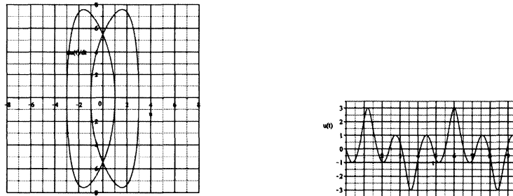
Figure 4.2: (left):The “triple-time oscillations” orbit with the initial condition: u(0) = 0, \dot{u}(0) = -\sqrt{30} in Example 4.1. \omega \doteq 4.808 . (right): The time history of the “triple-time oscillations” orbit. The time is shown up to two periods.
