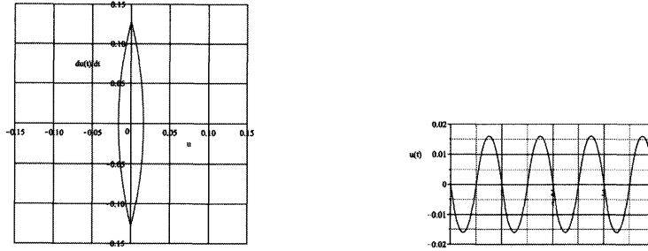
Figure 3.3: (left):The \omega(=1) -periodic orbit with the initial condition: u(0) = 0, \dot{u}(0) = \frac{\cos \frac{1}{2} - 1}{2 \sin \frac{1}{2}} = -0.1276709606\dots in Example 3.2. (right):The time histories shown up to four periods.
