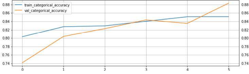
Figure 1: Training results on Melanoma detection with a new loss function without sigmoid activation, after 6 epochs.
