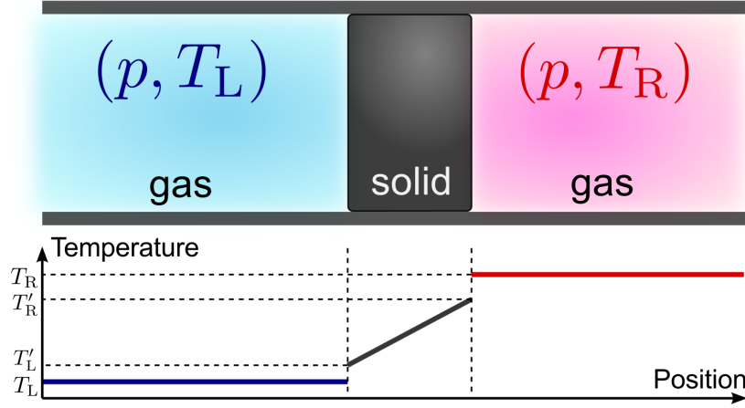
Fig. 4.1 Schematic illustration of the experimental systems. The solid separates two gases at the same pressure but different temperatures. The pressures and temperatures are kept constant over time. Temperature gaps appear on the solid surface.
