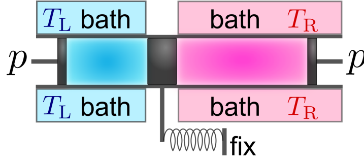
Fig. 4.5 Two heat baths are in thermal contact with two dilute-gas regions, respectively. The solid material is immobilized by a spring. F_{\text{gap}} can be measured in the experiment, while the steady-state motion is not observed.
