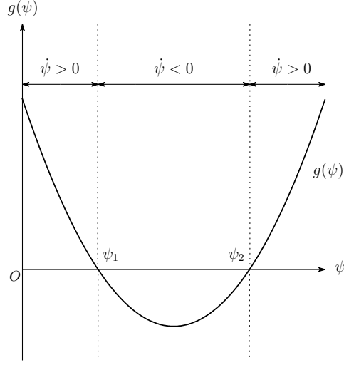
Fig. 2. Dynamics of \psi
