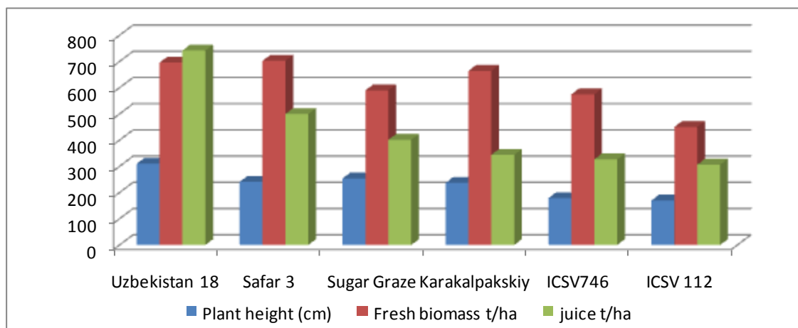
Fig. 2 Plant height, stalk yield and juice values of sweet sorghum
