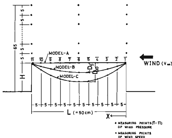
Fig. 2. Schematic of roof models and measuring positions (unit cm).
