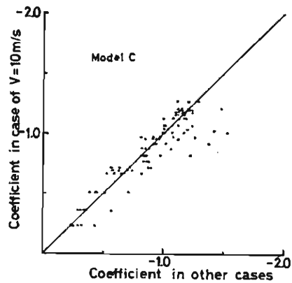
Fig. 18. Variation of pressure coefficient with wind speed (Model-C).
