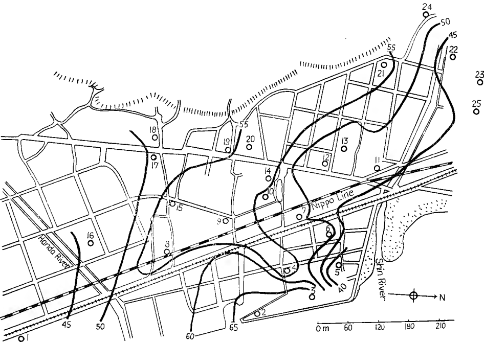
Fig. 1. Map showing temperature of spring water in Kamegawa, Beppu City, December 26, 1964. (in °C)
