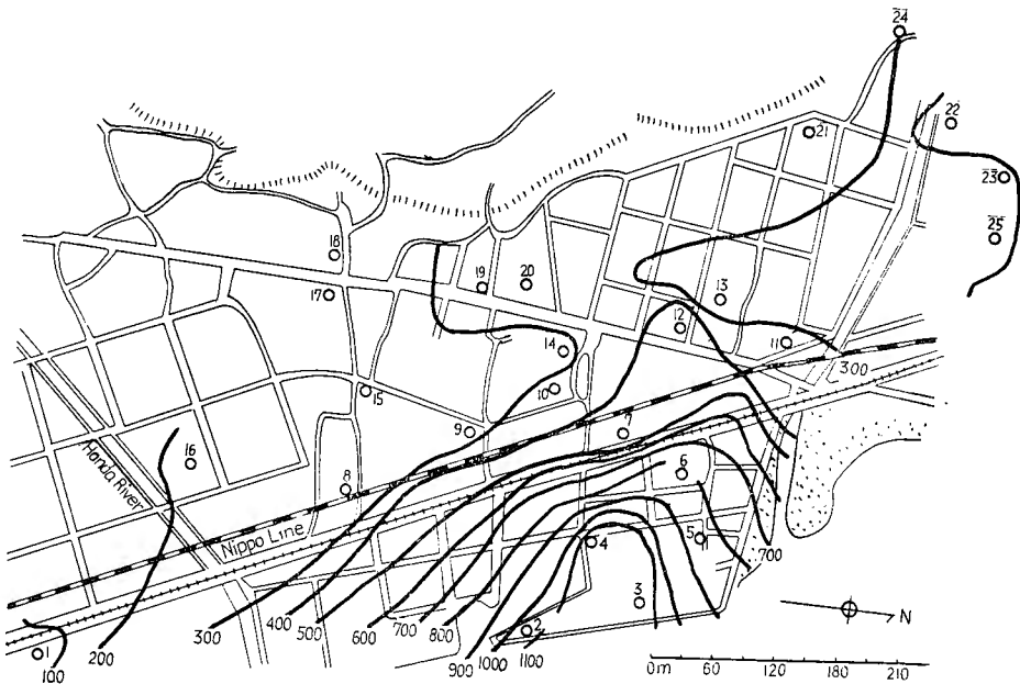
Fig. 2. Map showing distribution of chlorine ion concentration in Kamegawa, Beppu City, December 26, 1964. (in mg/l)
