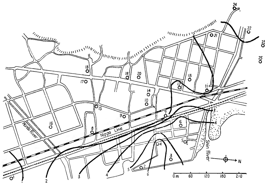
Fig. 4. Map showing distribution of calcium+magnesium concentration in Kamegawa, Beppu City, December 26, 1964. (in mm/l)
