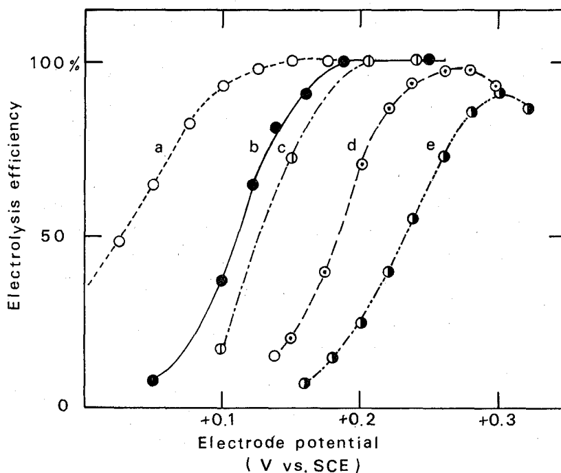
Fig. 3. Potential dependence of the electrolysis efficiency of bromide and chloride ions.
