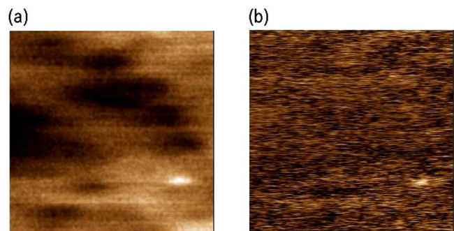
FIG. 4. (Color online) A confined submicrometer emission center seen in the near-field photoluminescence map (a) and the simultaneously taken polarization properties map (b). Image size is 3.75 \times 3.75 \mu\text{m} composed of 256 \times 256 pixels.
