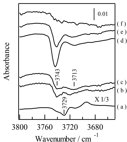
Figure 14. FT-IR spectra of \text{Nb}_2\text{O}_5/\text{Al}_2\text{O}_3 calcined at 1123 K with various \text{Nb}_2\text{O}_5 loadings. (a) \gamma\text{-Al}_2\text{O}_3 , (b) 5 wt%, (c) 14 wt%, (d) 16 wt%, (e) 18 wt%, (f) 30 wt% \text{Nb}_2\text{O}_5 loading.
