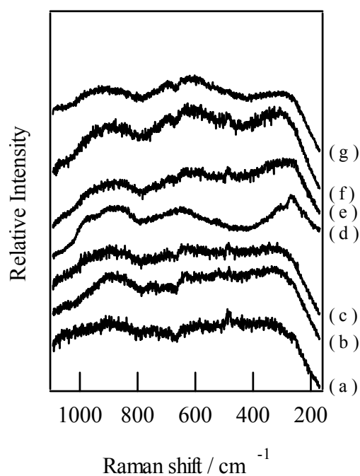
Figure 8. Raman spectra of \text{Ta}_2\text{O}_5/\text{Al}_2\text{O}_3 catalysts with various loadings. (a) 10 wt%, (b) 20 wt%, (c) 30 wt%, (d) 33 wt%, (e) 35 wt%, (f) 40 wt%, and (g) 50 wt%. Calcination temperature: 1223 K,
