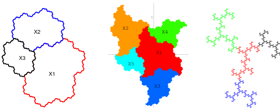
Figure 2. Rauzy fractals of irreducible type, reducible type and non-Pisot type. Left: Rauzy substitution (Example 3.1). Middle: Hokkaido substitution (Example 3.2). Right: A non-Pisot substitution (Example 3.3).
