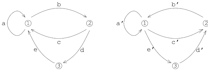
Figure 1. Left: Graph of IFS (2.4) in Example 2.3. Right: Reverse graph.
