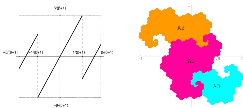
Figure 3. Left: Minimal weight transformation M_\beta (Example 4.6). Right: The invariant sets of the dual system of M_\beta .
