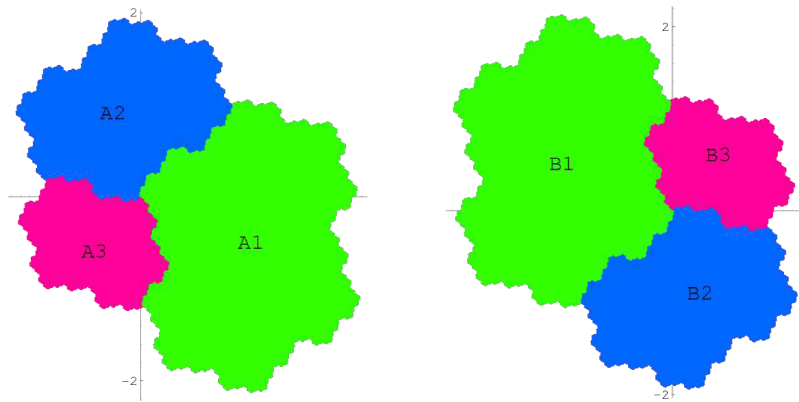
Figure 6. Invariant sets of dual system of symmetric \beta -transformation.
