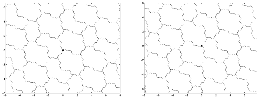
Figure 4. The Rauzy-Thurston tiling of symmetric \beta -transform has two pages for \beta : \beta^3 = \beta^2 + \beta + 1 . ([28]). See also Example 4.5 and Section 8.2.
