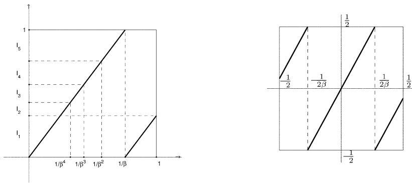
Figure 5. Left: \beta -transformation system with \beta^3 = \beta + 1 . Right: Symmetric \beta -transformation with \beta^3 = \beta^2 + \beta + 1 .
