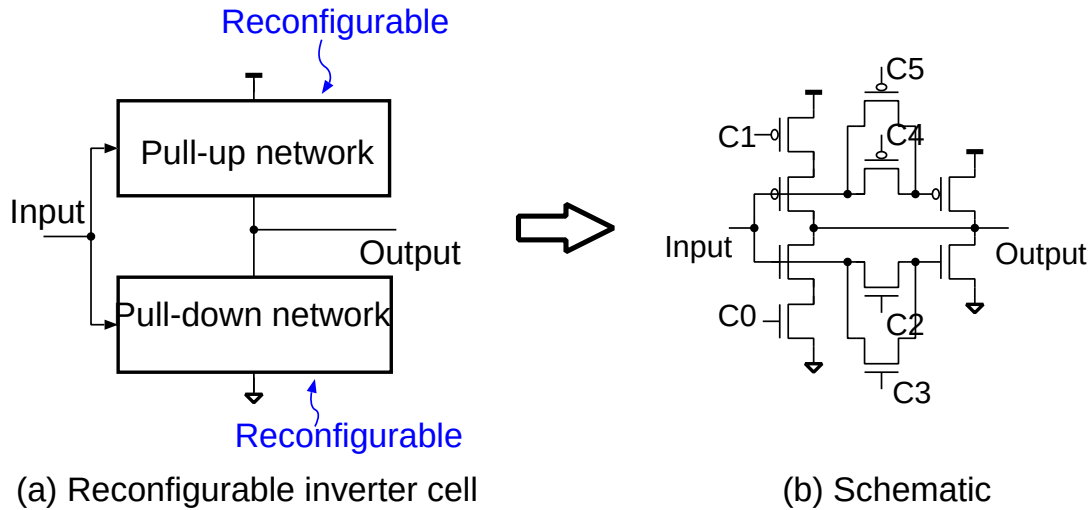
Figure 4.12: (a) Design of a reconfigurable inverter cell. Pull-up and pull-down networks are reconfigurable separately. (b) One design example of a reconfigurable inverter cell and its transistor level schematic. Various delay modes are realized. (©2014 JJAP)
