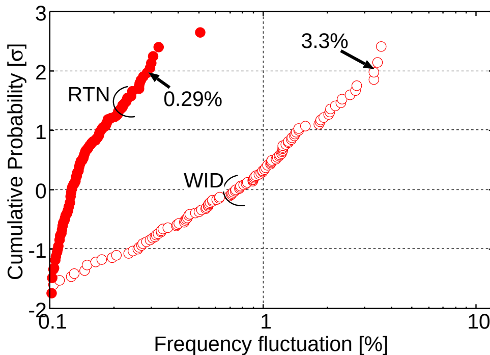
Figure 4.33: Comparison between RTN-induced frequency fluctuation and static process variation induced frequency fluctuation for pMOSFET. (©2014 JJAP)
