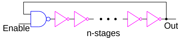
Figure 4.9: Schematic of ring oscillator circuit used for variation characterization. Conventionally, the inverter structure of each stage is fixed. Multiple ROs with different inverter structures are implemented for extracting various variation information.
