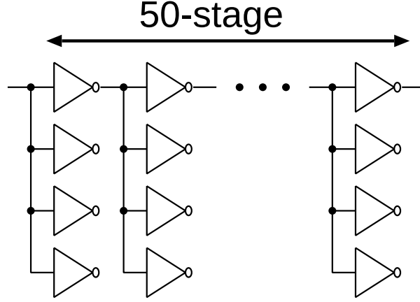
Figure 5.1: Circuit model used for delay and energy calculation. 50-stage fan-out 4 inverter chain as the circuit model.
