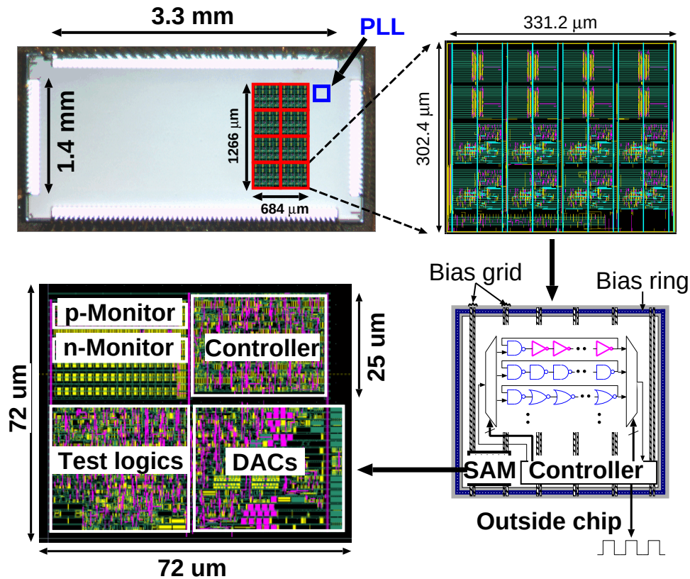
Figure 5.16: Chip photograph and layout of the self-adjustment scheme. ROs of several logic gates are implemented to evaluate critical path delays. (©2012 IEEE)
