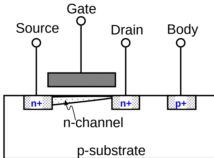
Figure 2.5: A cross section view of nMOSFET. Body terminal can be used as a forth terminal to tune the channel threshold voltage.
