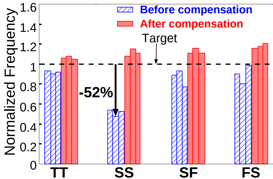
Figure 5.19: Frequencies of ROs consisting of various kinds of gates. INV, NAND and NOR frequencies are plotted for each corner from the left. (©2012 IEEE)
