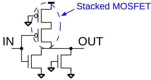
Figure 3.9: An inverter cell with stacked pMOSFETs (NOR2).
